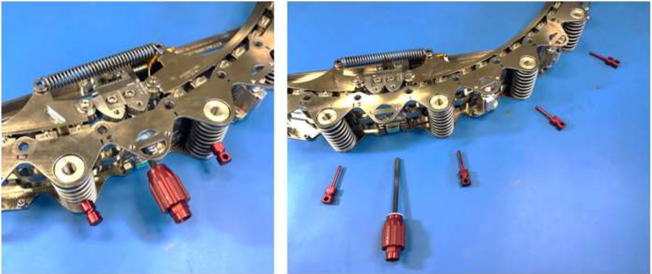
Figure 12-3: Removing the Stow Screw and Spring Locks
