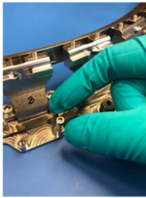
Verify screws and accepting threads are free-running
