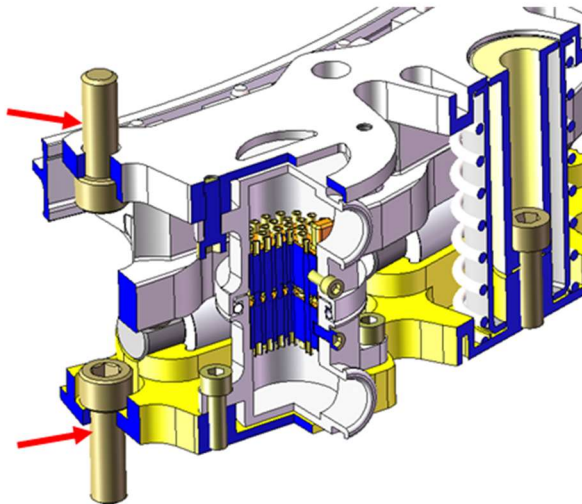
Figure 9-2: Fasteners and torques for adjoining structures
