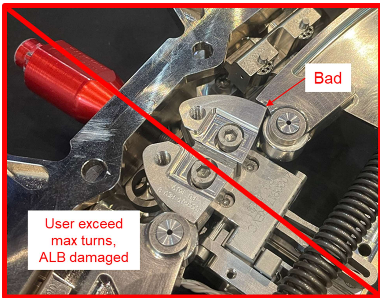
Figure 11-5: Over-stowed ALB
