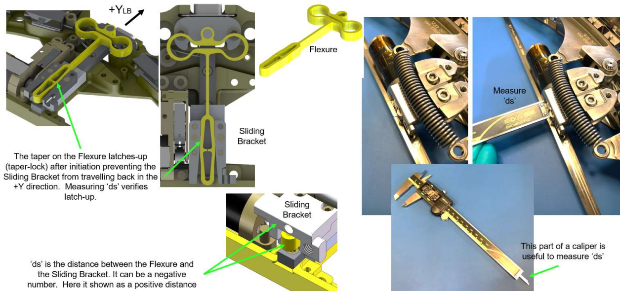
Figure 10-2: Measuring 'ds'
