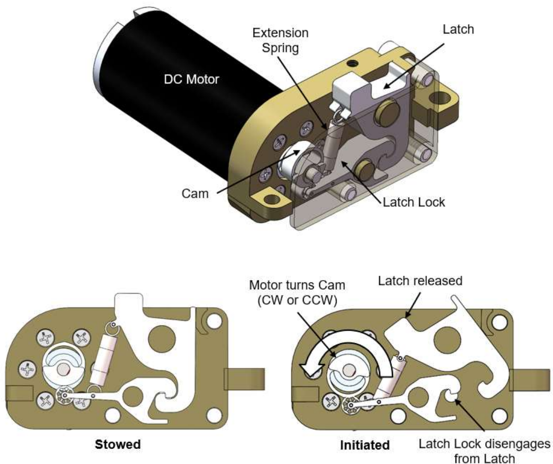
Figure 12-5: Powered Motor and initiation
