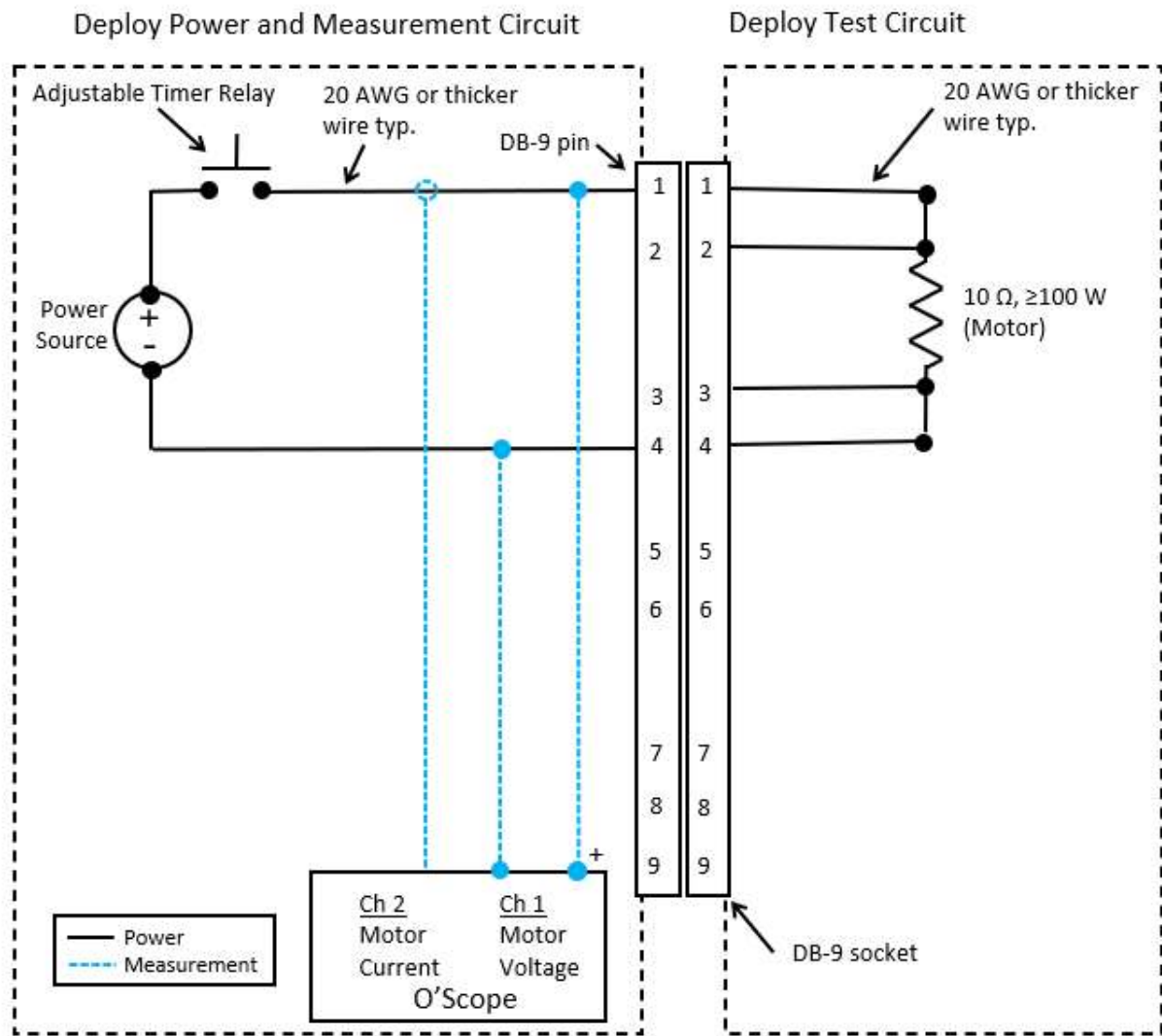
Figure 12-1: Deploy test circuit
