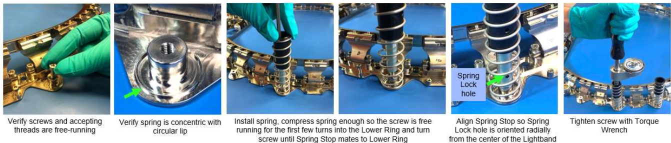
Figure 8-3: Attaching Separation Springs
