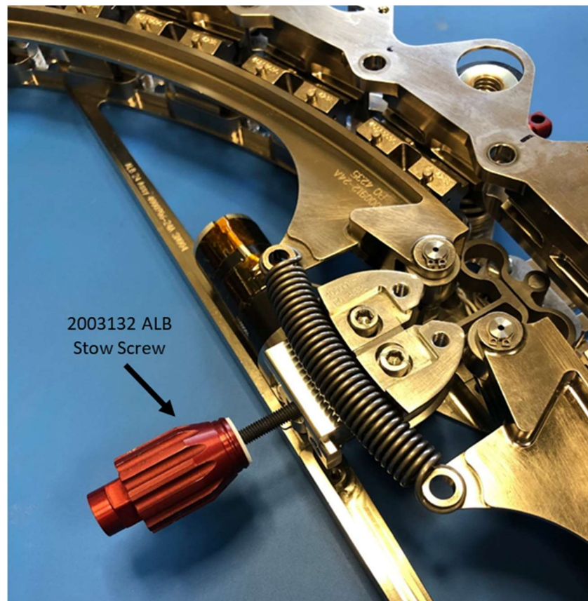
Figure 10-3: The quality of the threaded junction is verified by turning the Stow Screw into the Sliding Bracket from the inside (not enough room on ALB8 for this operation)
