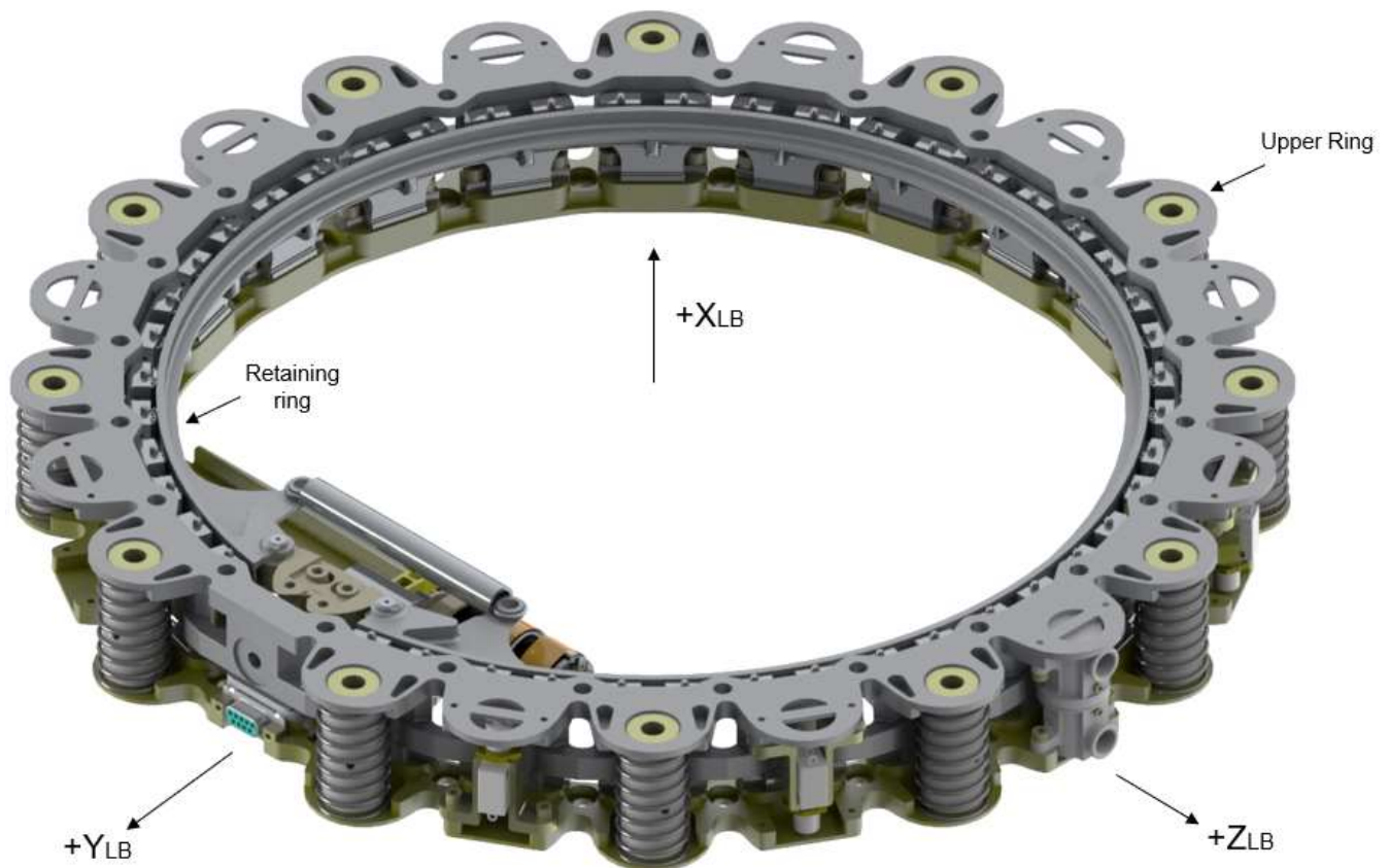
Figure 3-1: ALB15.000-24, Stowed
