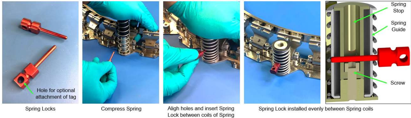
Figure 10-1: Installation of Spring Locks
