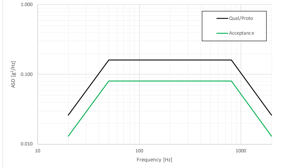
Figure 7-2: Random Vibration Testing
