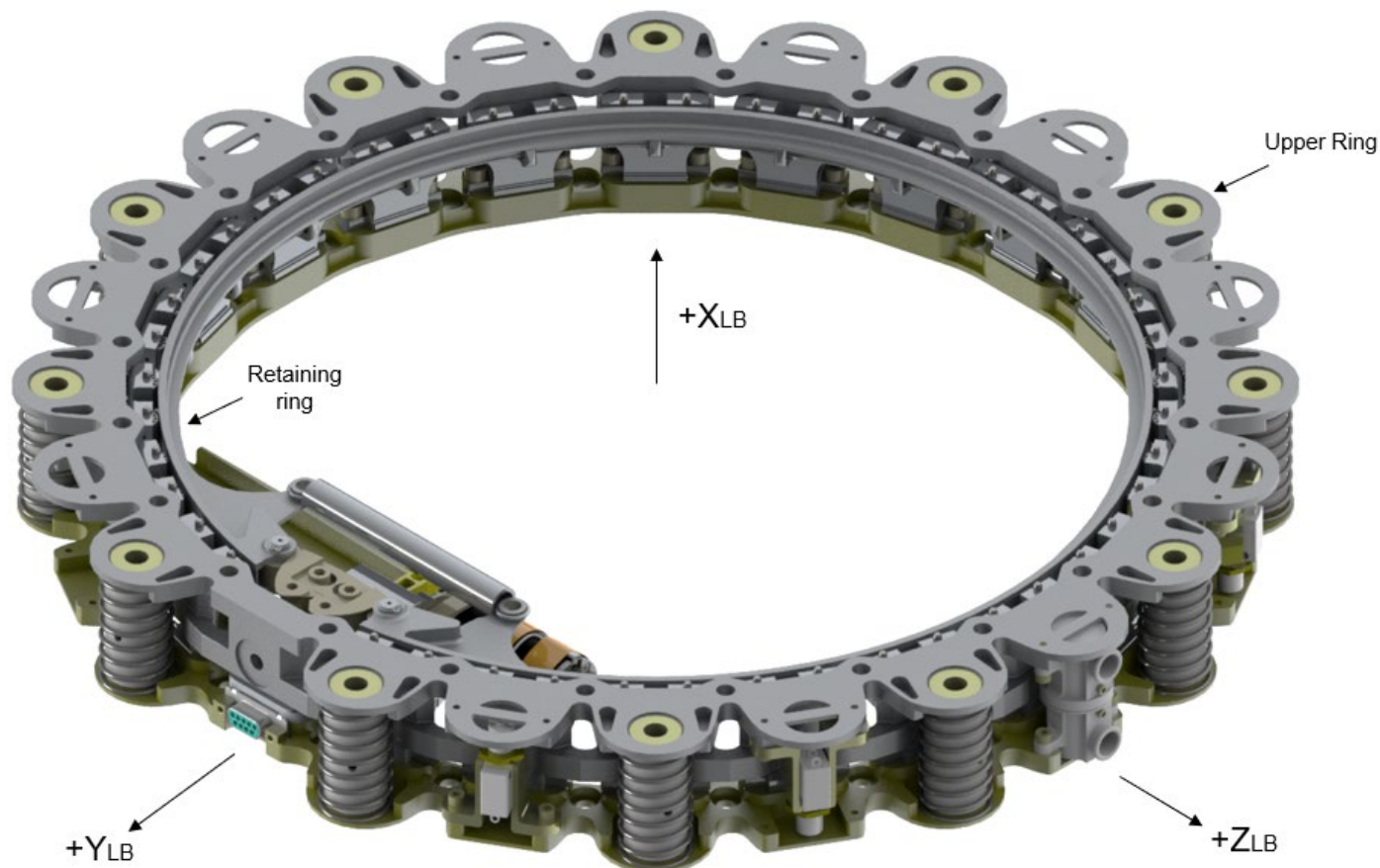
Figure 4-1: Stowed ALB
