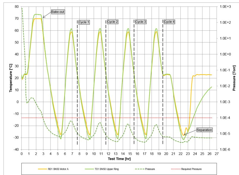
Figure 7-3: TVAC Testing
