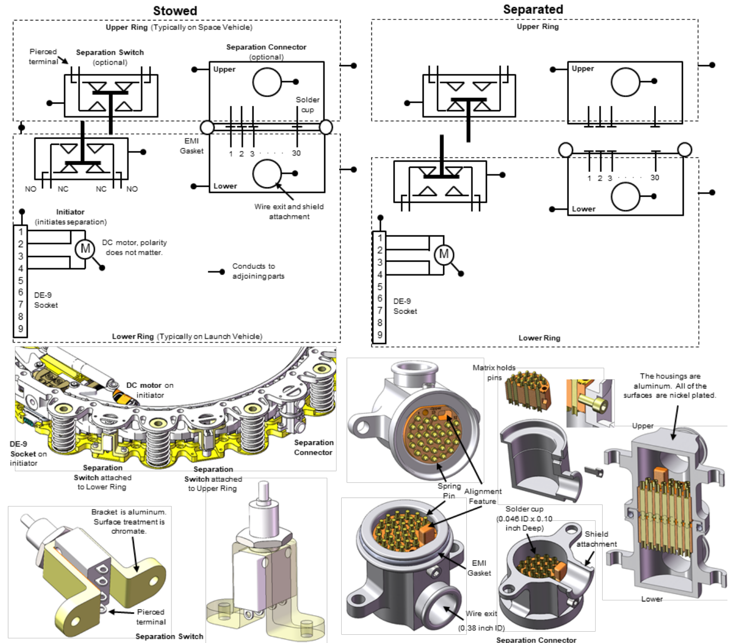
Figure 4-4: Schematic
