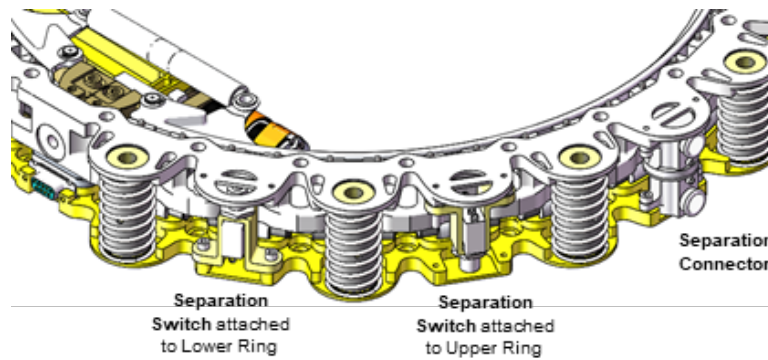
Figure 14-1: ALB Accessories
