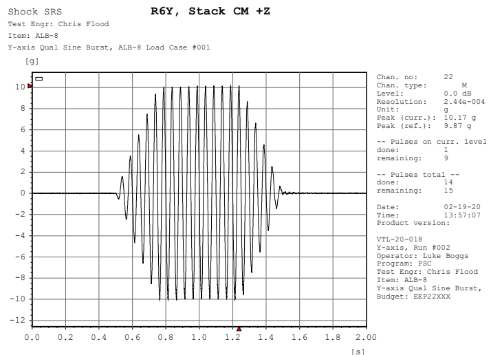
Figure 7-7: Fatigue Testing
