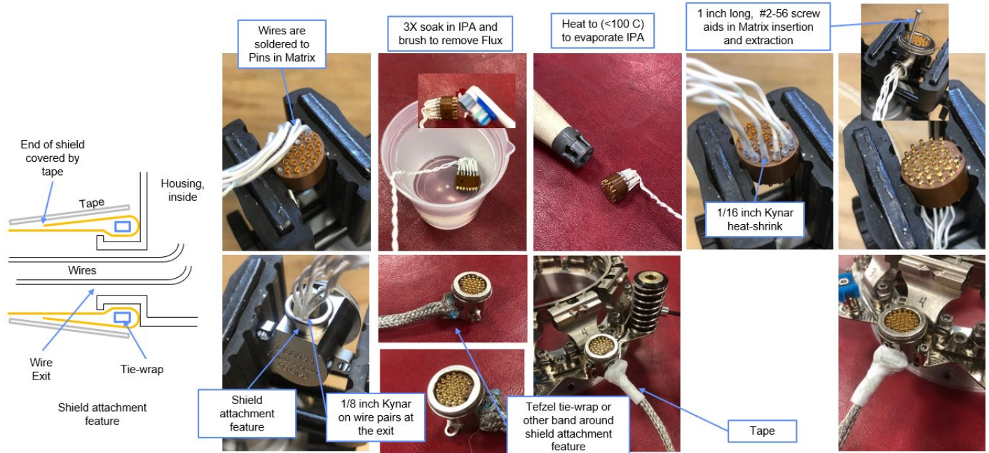
Figure 144-5: Wiring of Separation Connector
