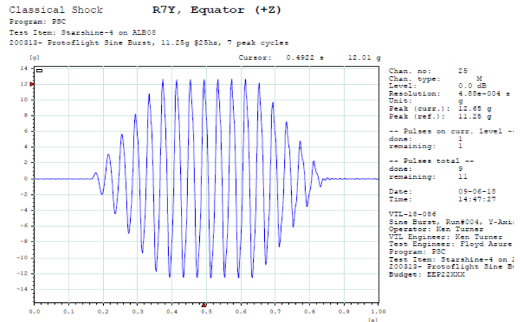
Figure 7-6: Strength Testing
