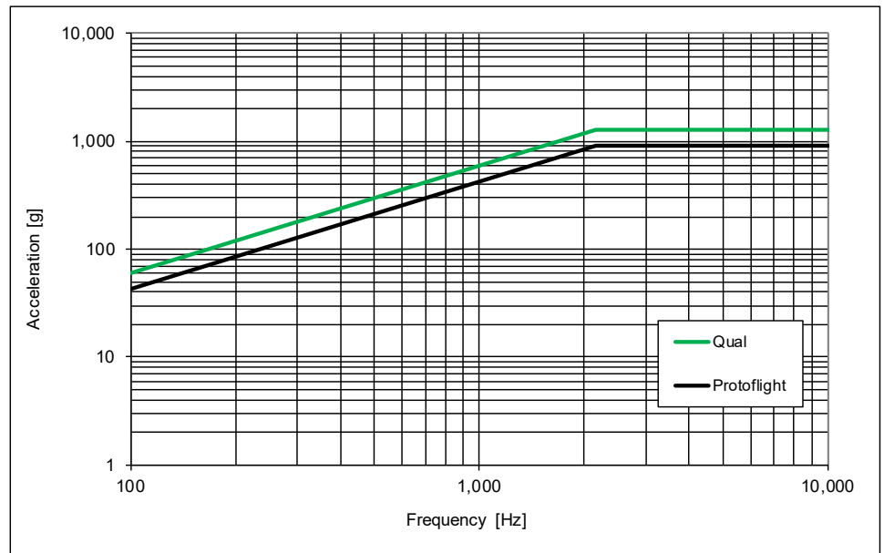
Figure 7-4: Shock Testing
