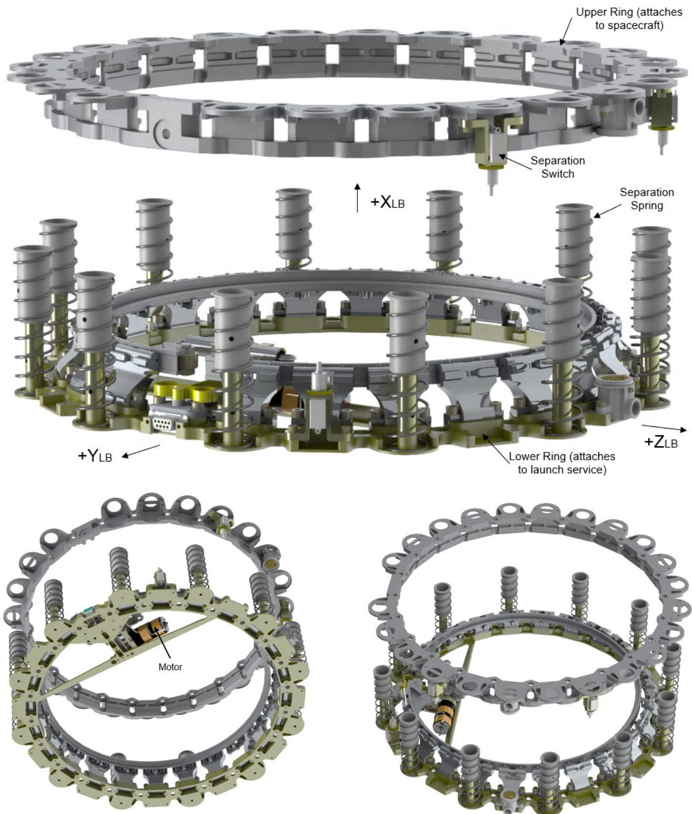
Figure 4-2: Separated ALB
