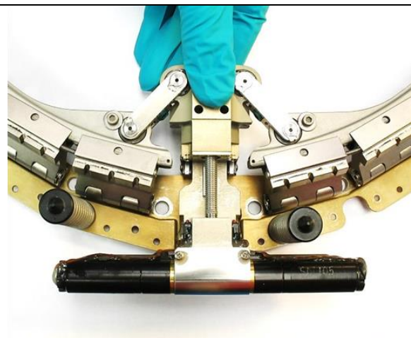
b) Correct position (Deployed)
