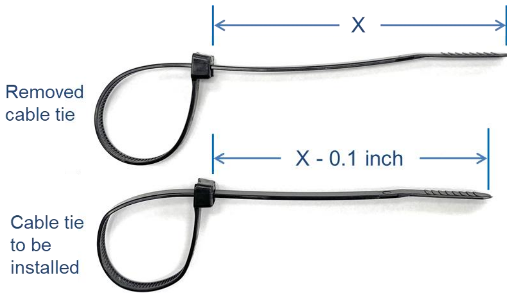
Figure 18-4: LCT reversal length
