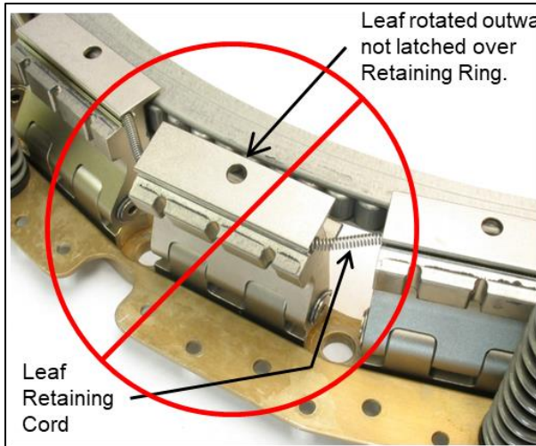
a) Incorrect Leaf position.
