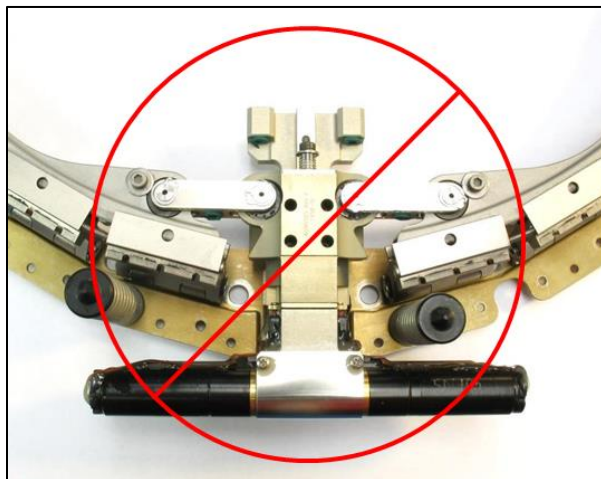
a) Incorrect position (Stowed)
