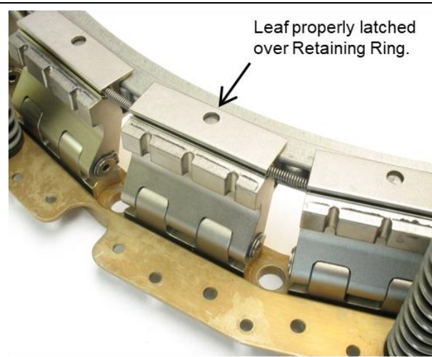
b) Correct Leaf position.
