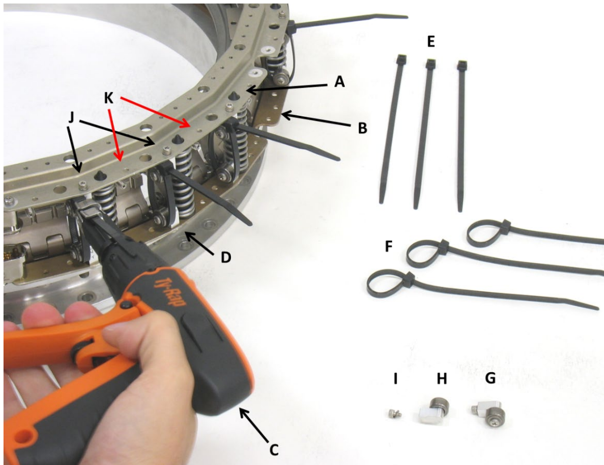
Figure 18-1: LCT Equipment
