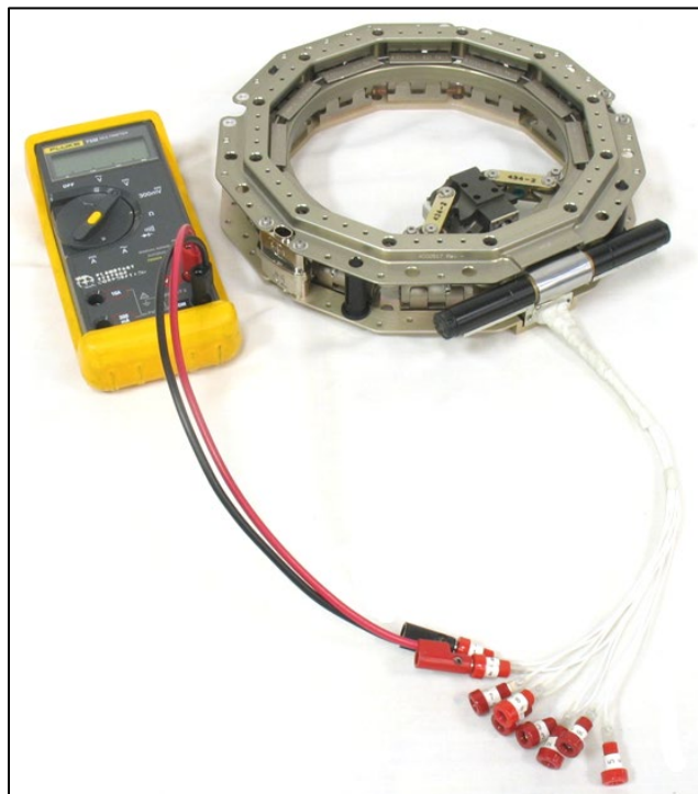
Figure 16-2: DMM and DB-9 breakout cable used to measure Motor Bracket Assembly resistance.
