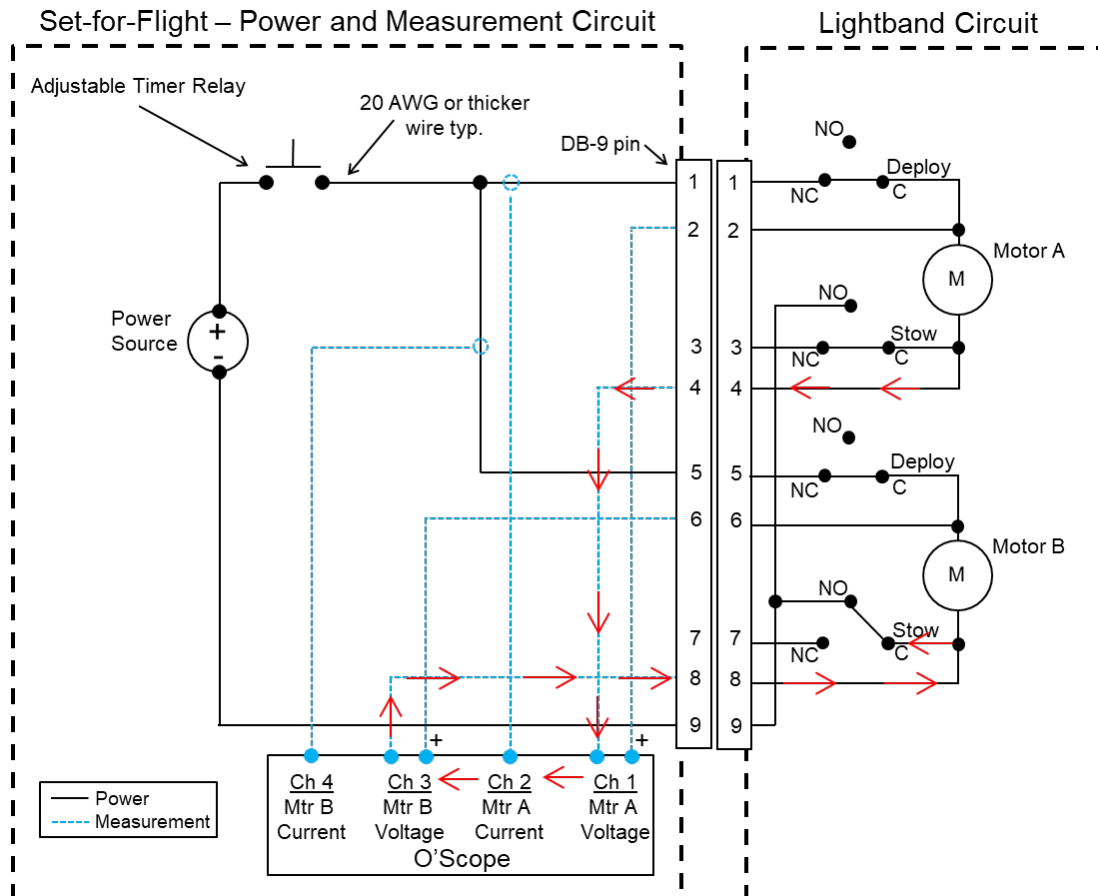
Figure 17-1: Set-For-Flight oscilloscope common probe warning
